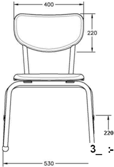
VISTA FRONTAL
