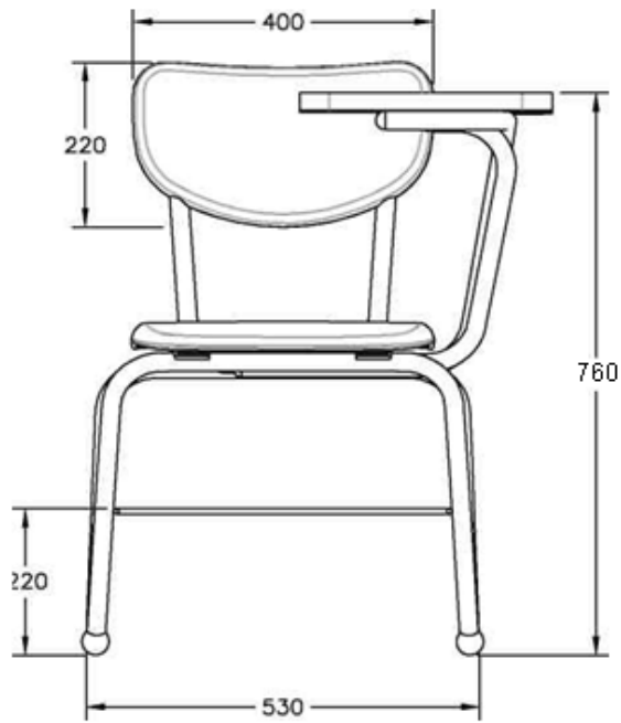
VISTA FRONTAL
