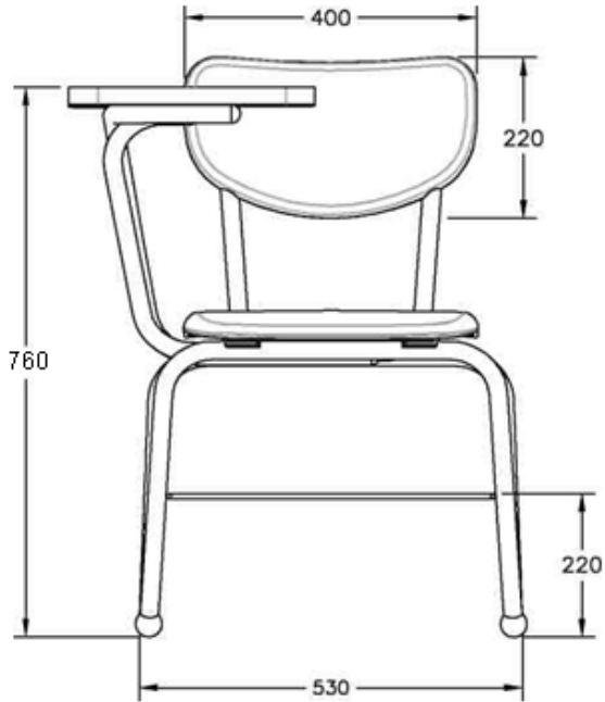
VISTA FRONTAL
